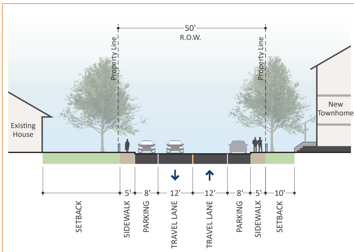
Figure 3-3: Neighborhood Streets Typical Proposed Section
