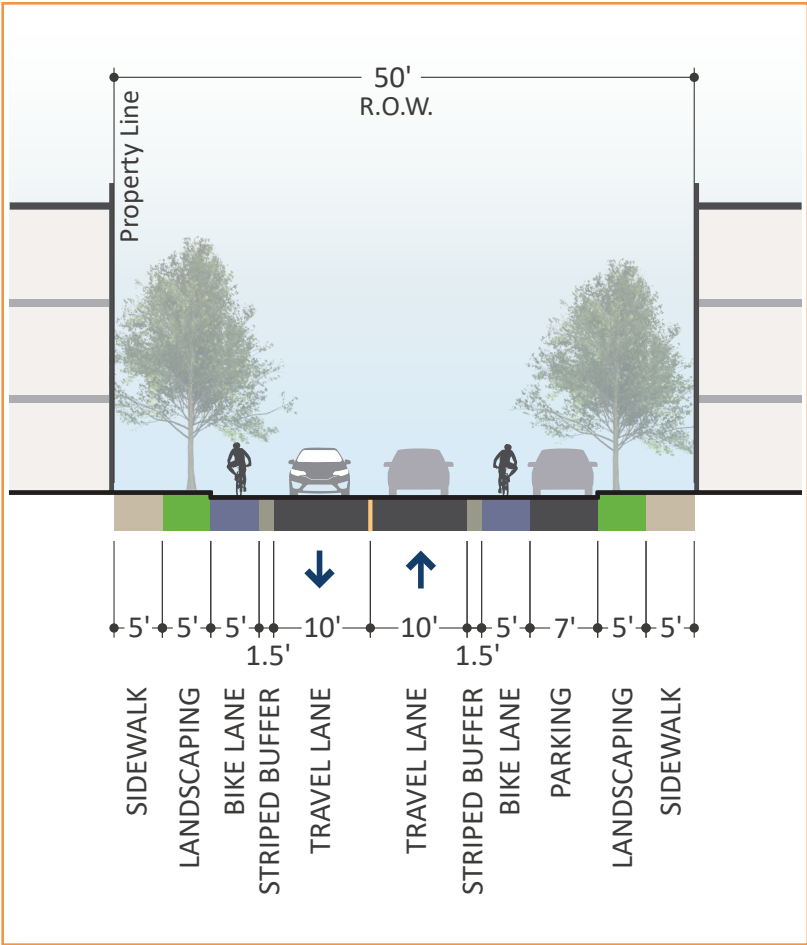
Figure 3-5: Harvey Avenue Extension Proposed Section
