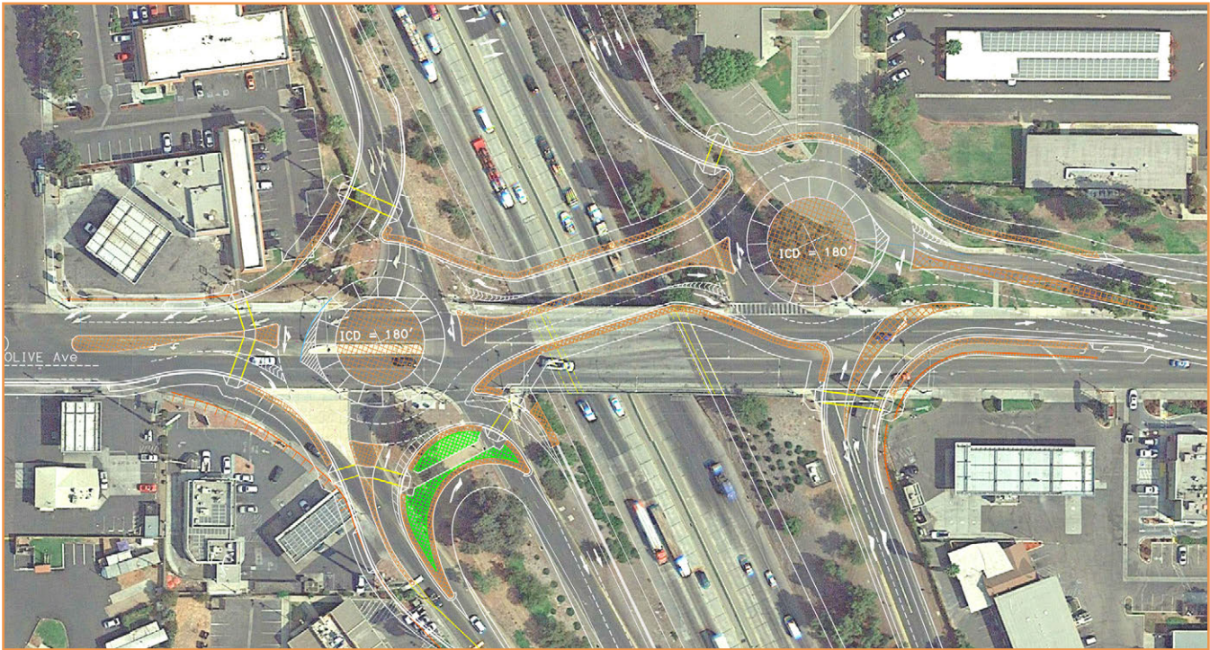
Figure 3-7: Proposed Caltrans Roundabout Design at Olive Avenue Source: Caltrans, 2022.
