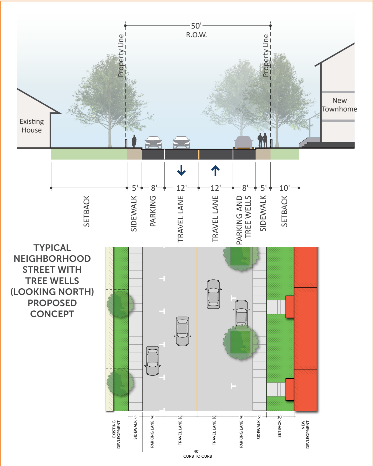
Figure 3-4: Neighborhood Streets Proposed Section with Tree Wells
