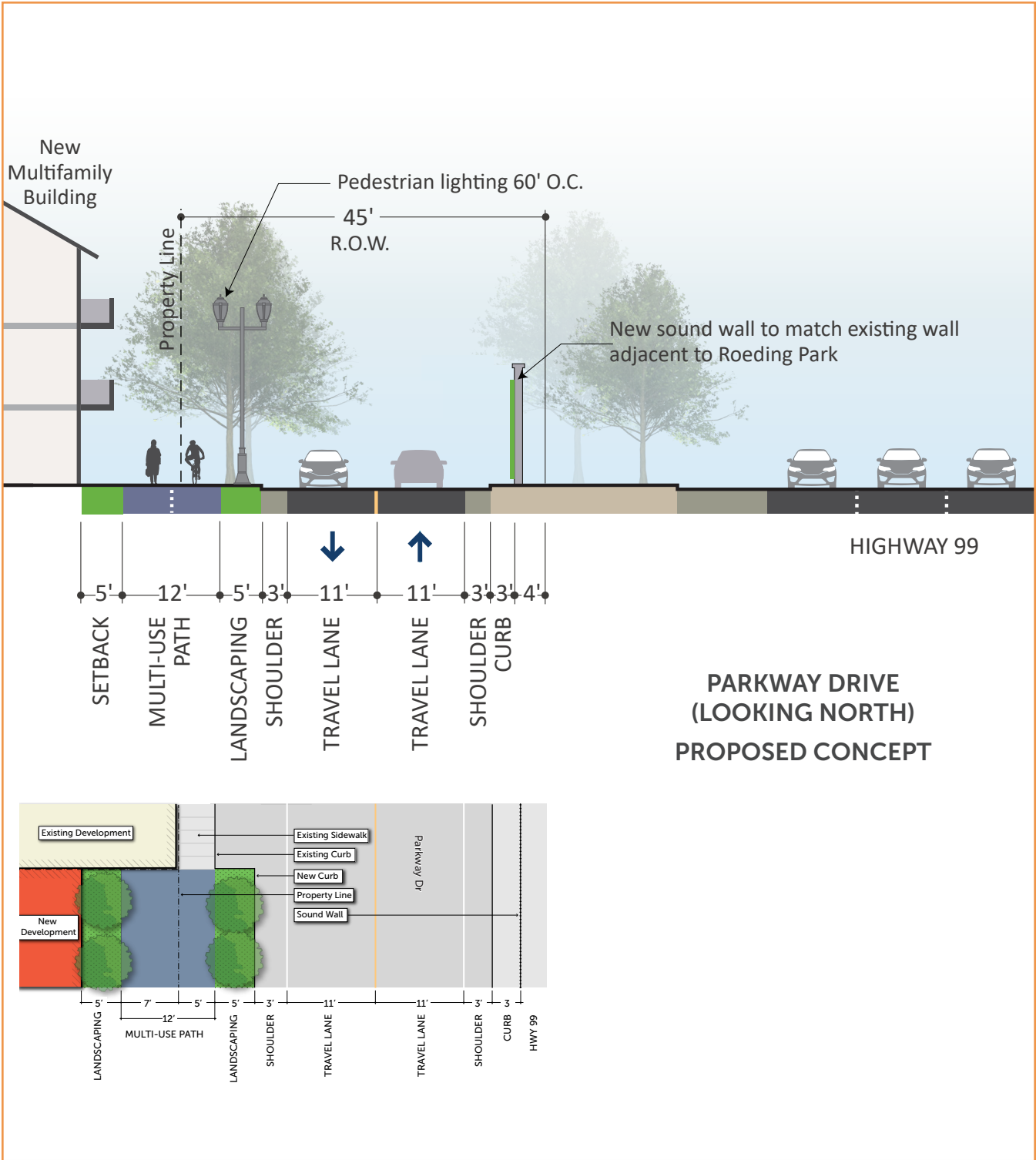
Figure 3-2: Parkway Drive Proposed Section
