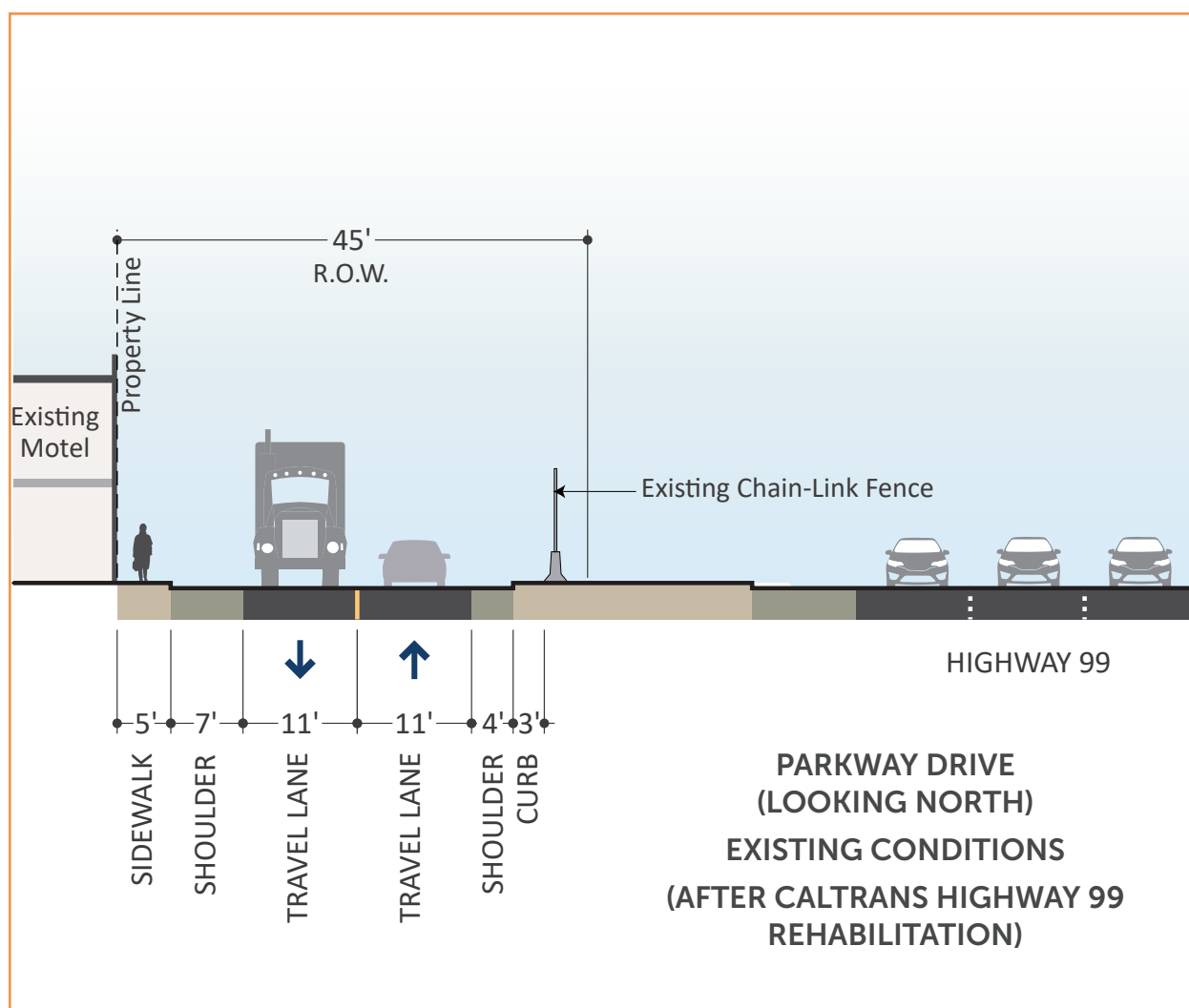
Figure 1-6: Parkway Drive Existing Section
