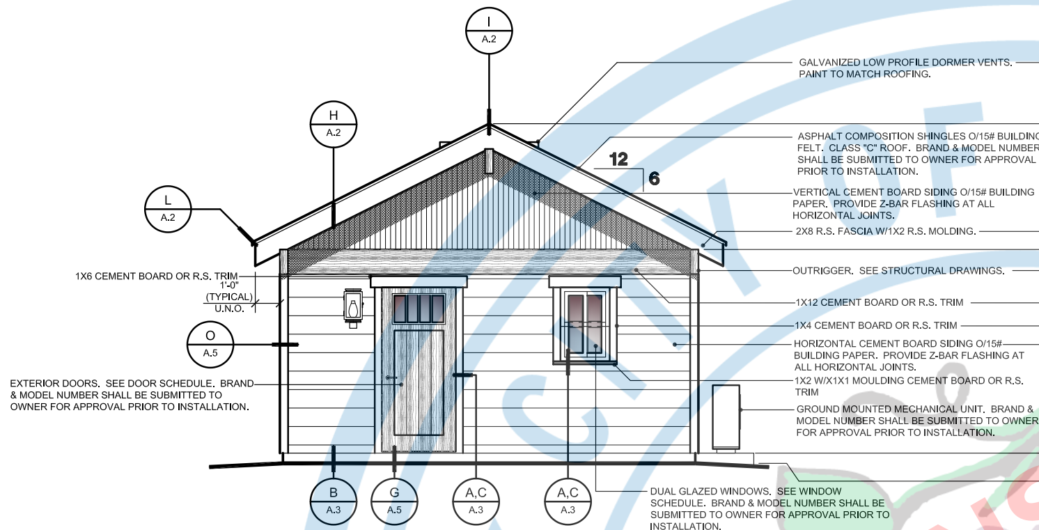
FRONT ELEVATION CRAFTSMAN MATERIALS AND SPECIFICATIONS ABOVE ARE APPLICABLE TO ALL SIDES OF THE ACCESSORY DWELLING UNIT.
