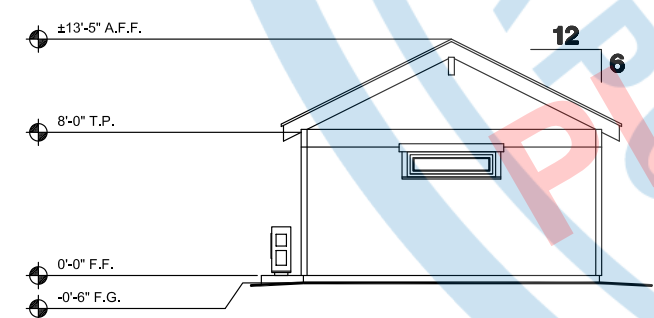
REAR ELEVATION CRAFTSMAN
