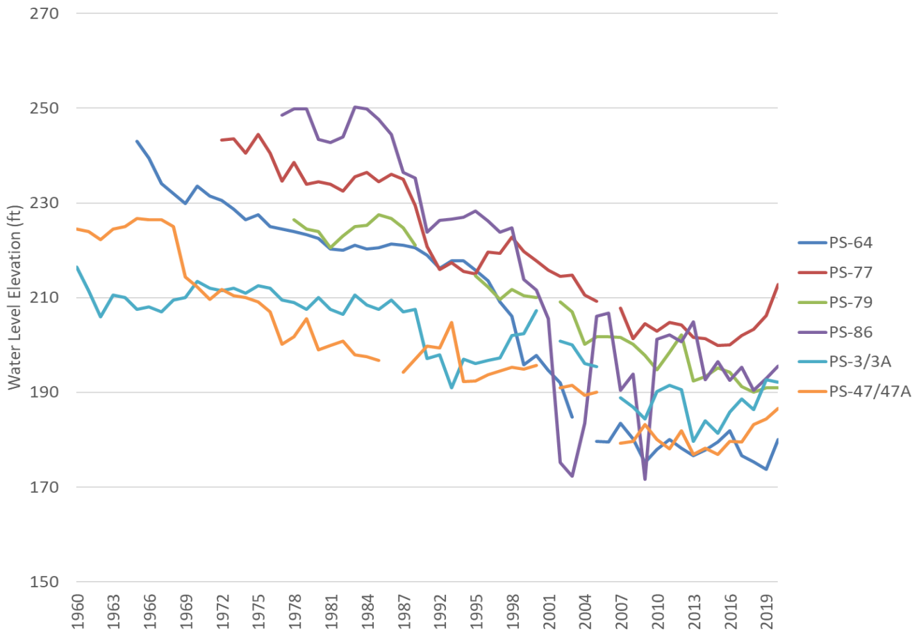
Figure 6-4. Time Series of Groundwater Levels at Representative Wells
