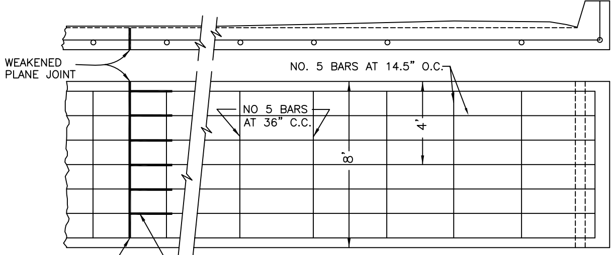
PLAN - SECTION
