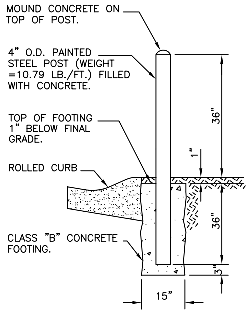
DETAIL OF STEEL GUARD POST
