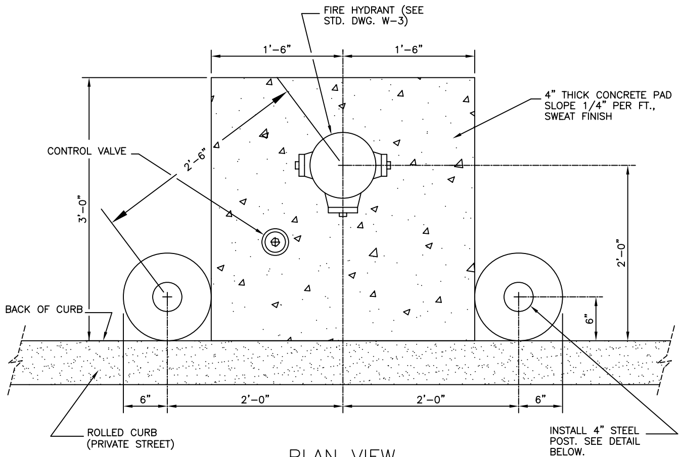
PLAN VIEW
